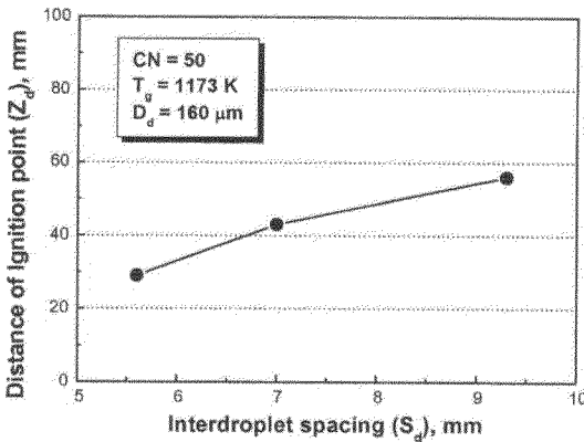
Fig. 5 Distances of ignition point with interdroplet spacing
