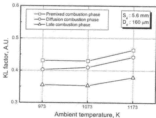
Fig. 8 Relation between KL factors and combustion phase with the ambient temperature
