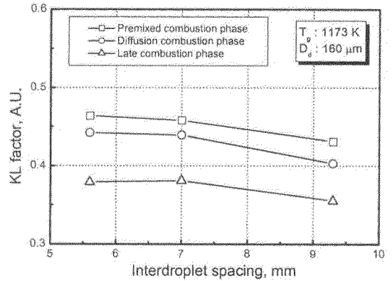
Fig. 10 Relation between KL factors and combustion phase with the interdroplet spacing
