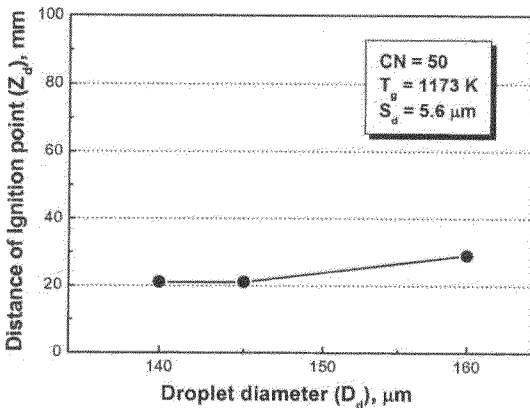
Fig. 6 Distances of ignition point with droplet diameter
