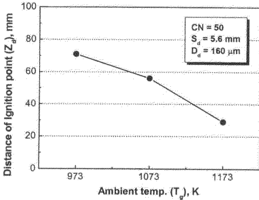
Fig. 4 Distances of ignition point with ambient temperature
